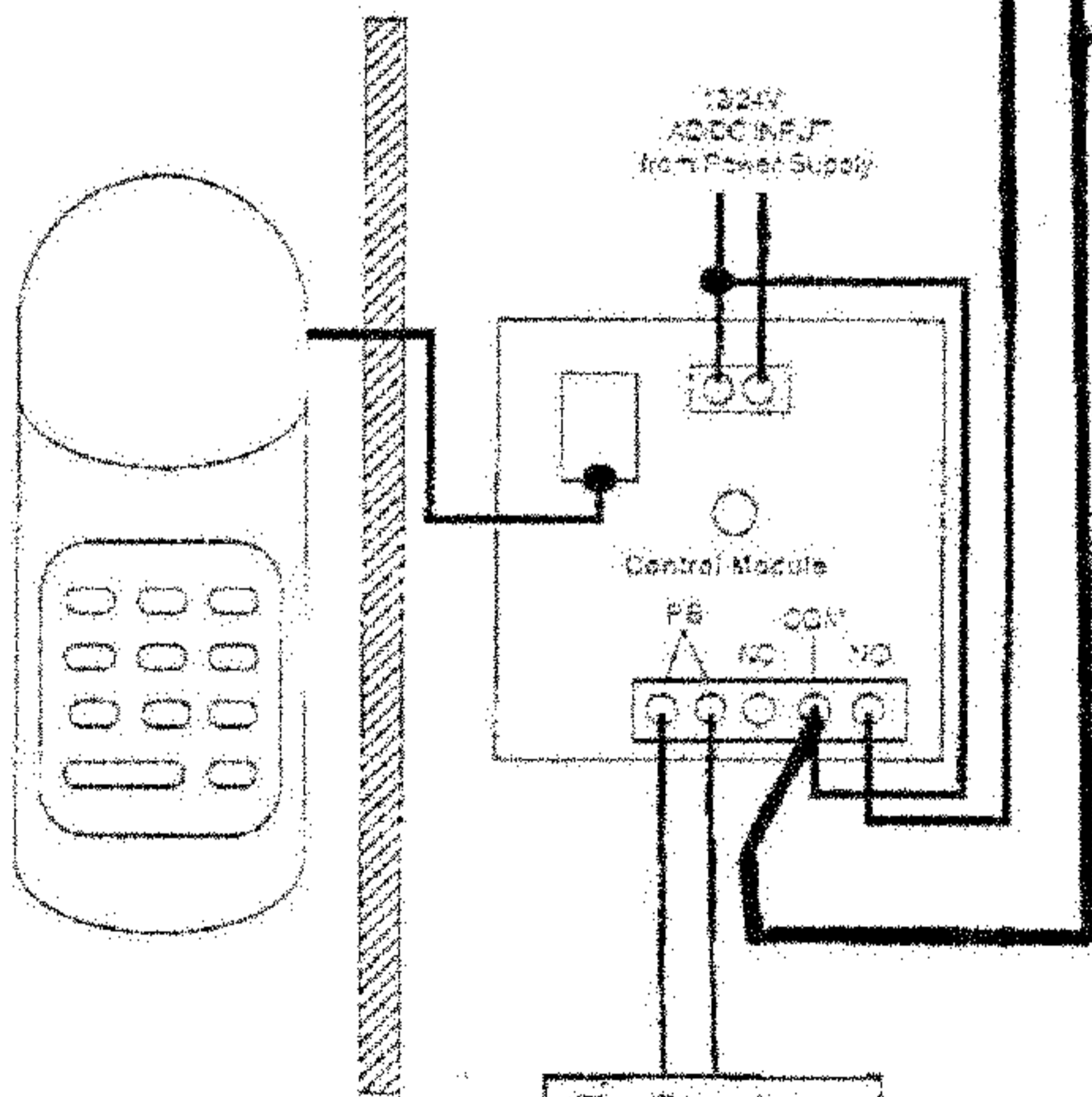
2nd Keypad and Control Module (Secondary)
