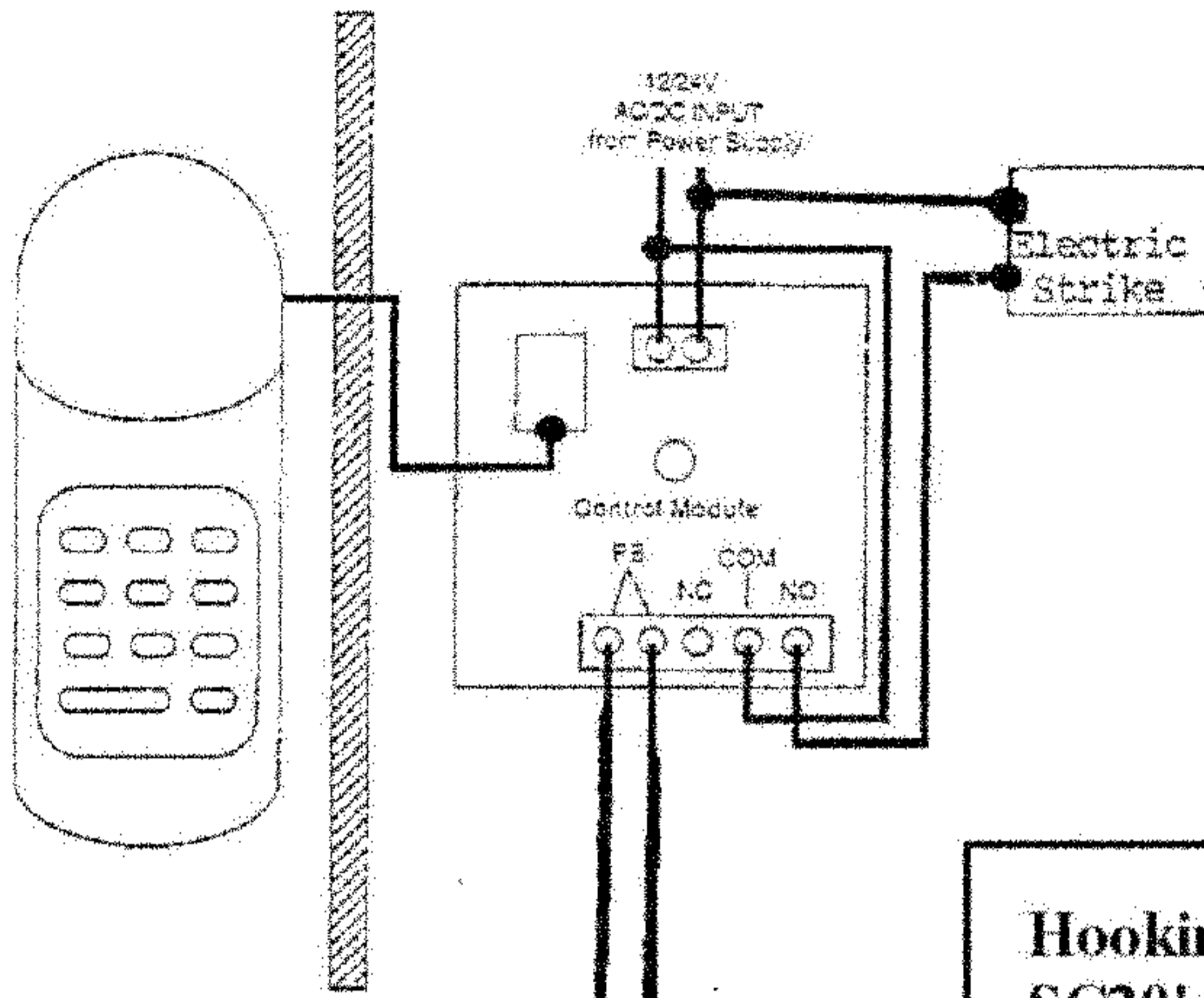
1st Keypad and Control Module (Primary)
